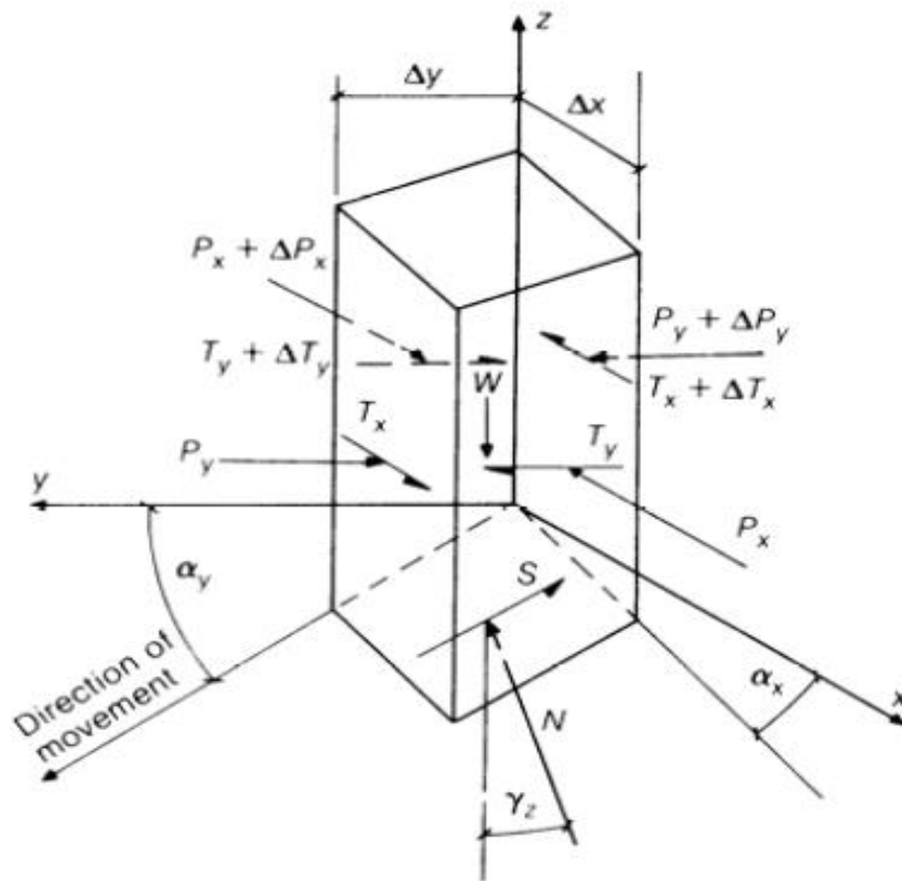
Figure 2-2: Forces acting on a single column (adopted from Hungr 1987).
